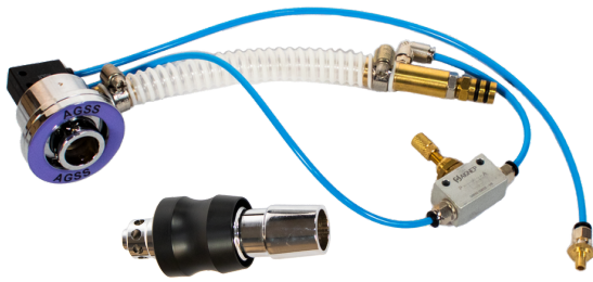
Agss Venturi - Agss venturi system
